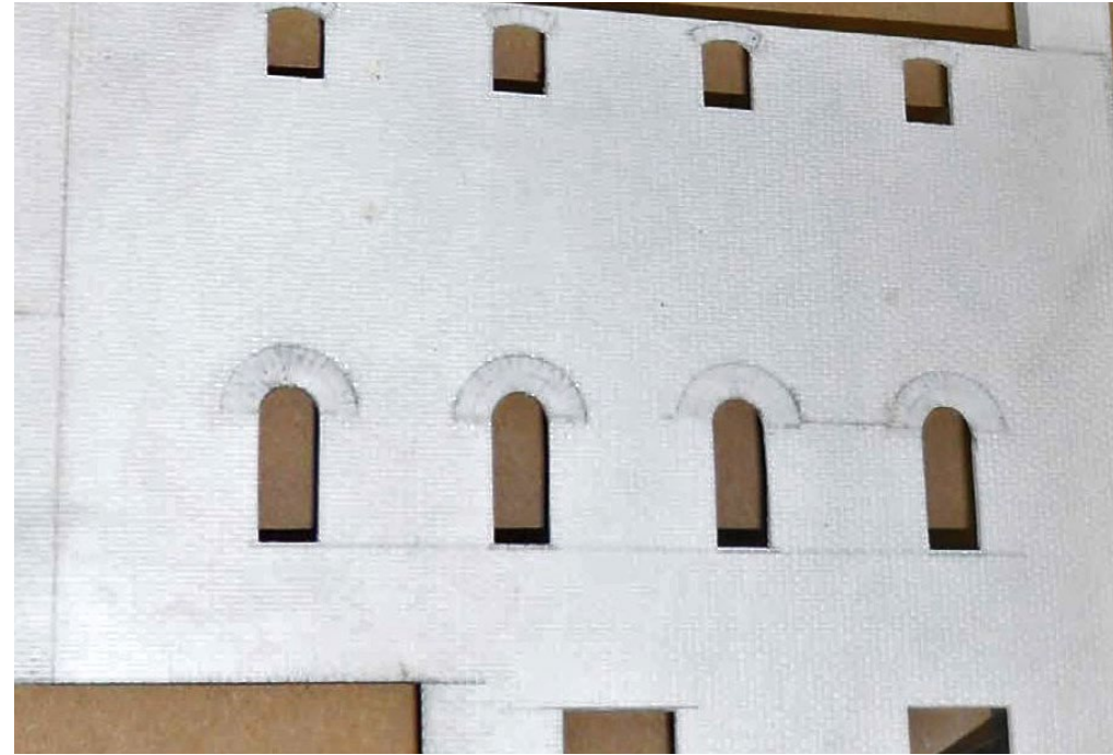
20. The brick header arches are added to the brick sheeting. The thickness of the material adds depth to the arches and helps them to stand out.
