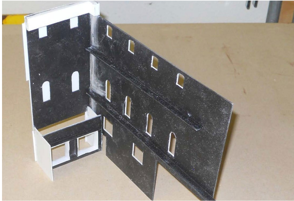
18. An inside view of the right wing. I added bracing to prevent warping of the sides. I also allowed for the bracing to overlap the joint between the sections to add strength to the structure.
