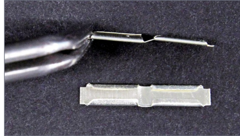
9. Specialized rail joiners from Atlas to connect code 100 to code 83 track.
