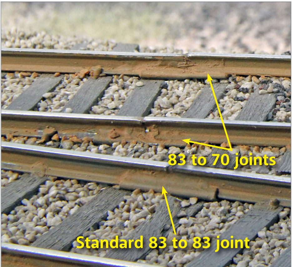
8. ME code 83 rail to code 70 rail joints using squished ME code 83 rail joiners, compared to a standard code 83 to code 83 joint.
