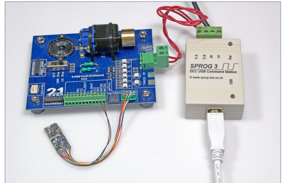
3. SPROG 3 connected to an ESU decoder tester and a LokSound Micro decoder.
