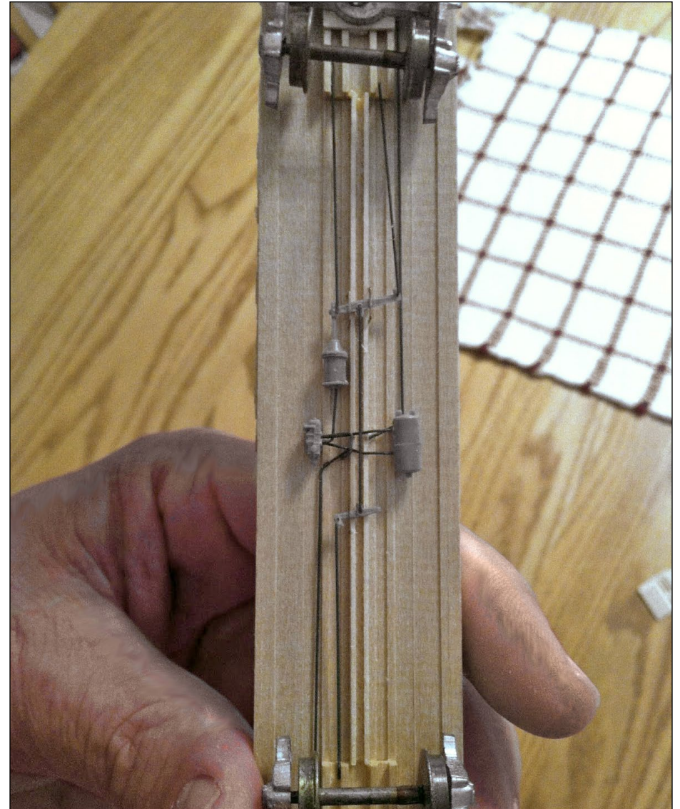
5. Add brake detail using the Tichy AB brake kit. Use soft floral wire for the piping. Because the picture of the boom car [1] is the only one known to exist and there are no known drawings of the brake rigging, we added the details to simulate the prototype as best we could.
