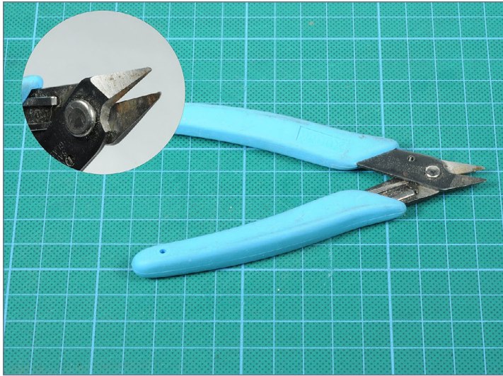
12. These Xuron 440 High Precision Scissors are perfect for cutting thin sheet brass and cutting photo-etched parts free from their fret.
