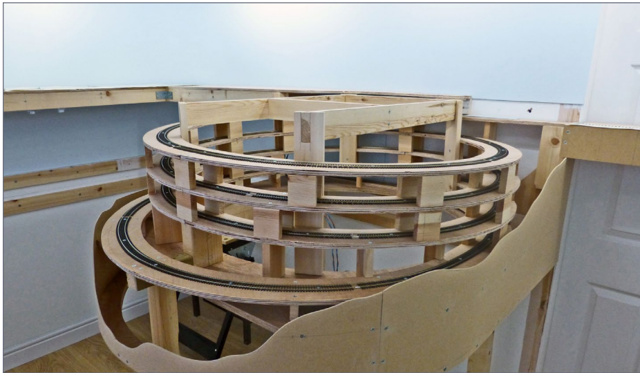
1. This is the starting point of the problem – a very ugly helix.
