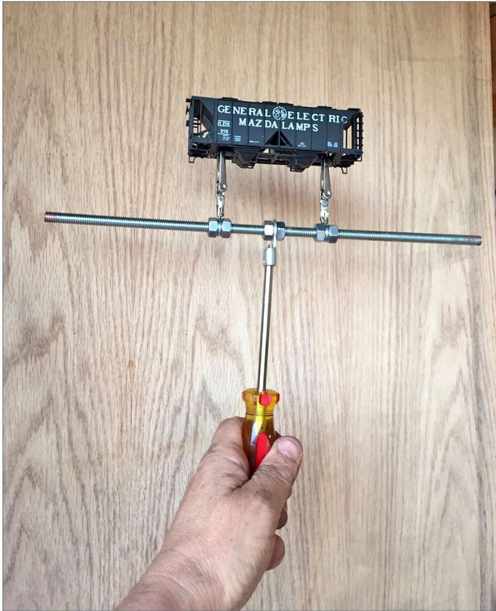
3. The completed painting handle with a Bowser two-bay covered hopper.
