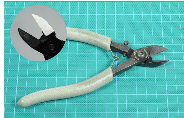
14. I replaced my economically priced flush cutters with these flush cutters from Rio Grande jewelry supply. Their large handles makes it easier to cut thick materials, but their use should still be limited to soft metals such as copper and brass.
