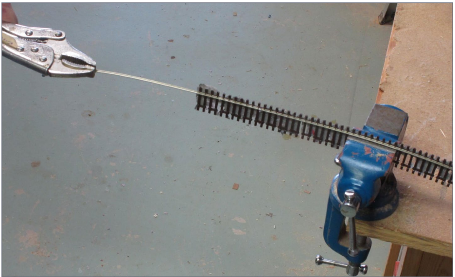
2. Pulling rail out of Atlas track.
