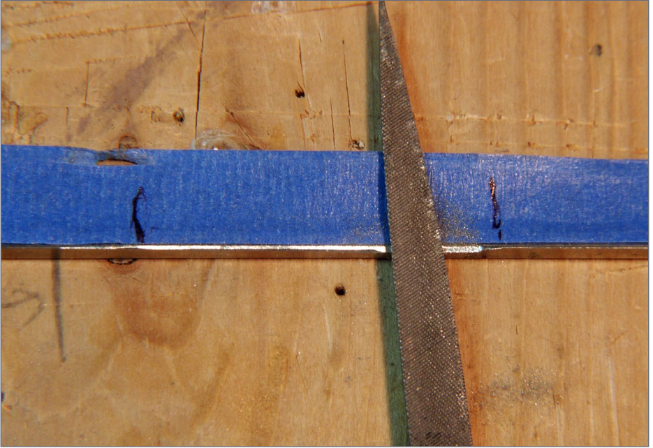
4. Final filing of the rail base in the stock rail.
