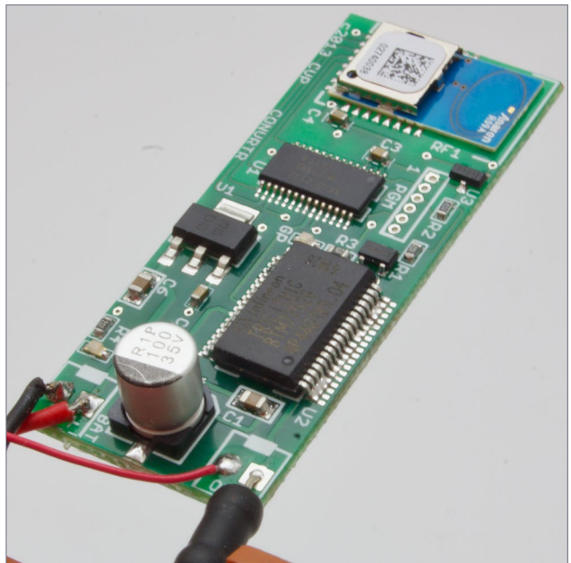
5. CVP CONVRTR-25 AirWire to DCC converter. The internal antenna is shown in the photo as the blue rectangle in the upper right. Bruce Petrarca photo
