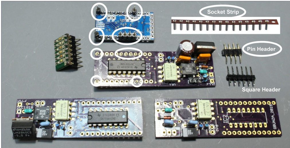
18. Socketed decoders.
