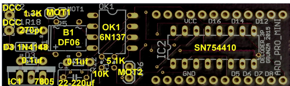
14. Top component placement.
