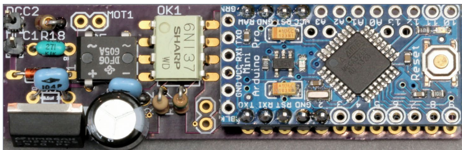
13. Top mounted decoder components.
