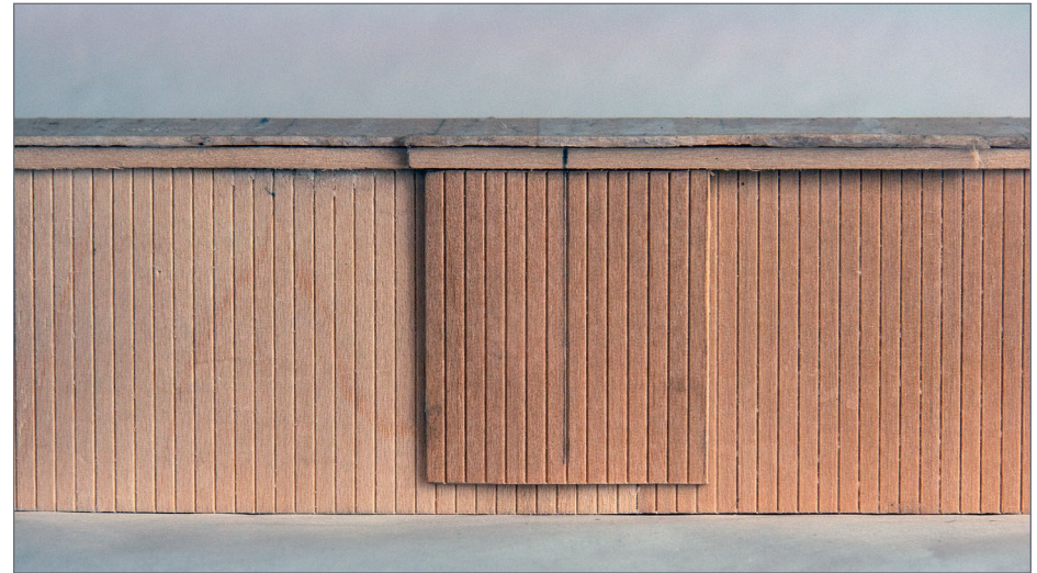
14. The door is cut from 1/32" x 3/32" scribed sheet. Center lines assist in aligning the door to the correct location on the track.
