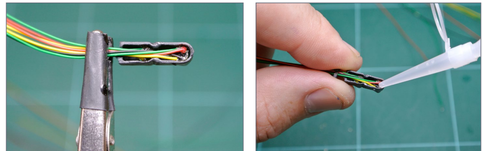
25. Installing the second LED.
