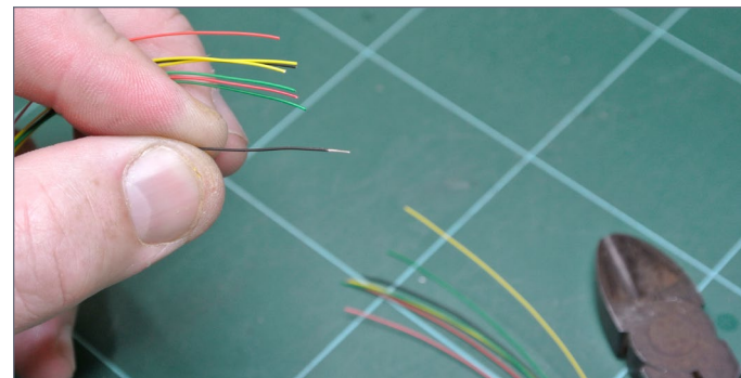
13. Wire with sheath removed and tinned.
