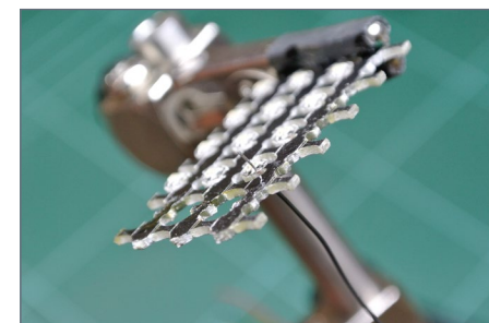
14. LED PCB and pads with wire through a pad hole.
