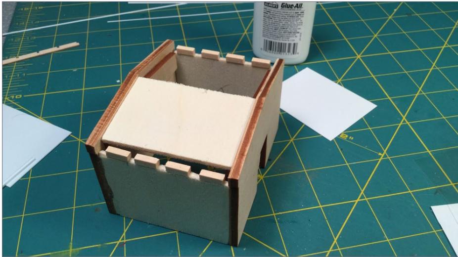
13. My third model of the oil house under construction. The basic “box” is 1/8” birch plywood. The laser-cut sides produced by Monster Modelworks include cut-outs for the I-beam roof supports.
