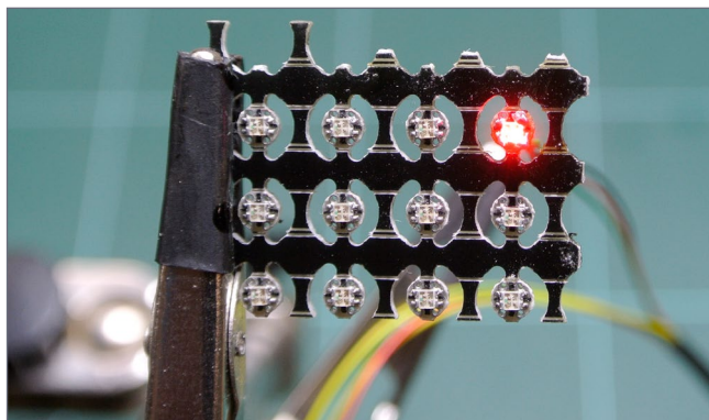
16. Testing the LED color while it's still part of the PCB array.
