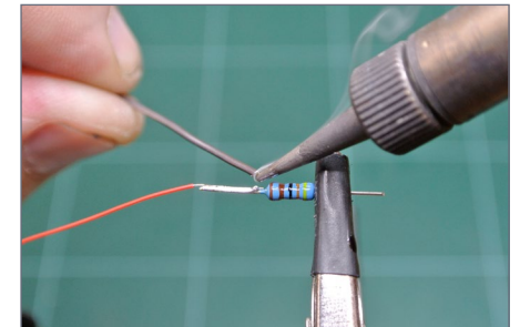
28. Resistors I use, and soldering the resistors to the LED lead wire.
