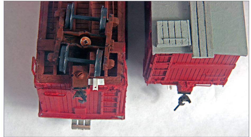
38. A short length of .100" channel has been drilled and glued to the .020" x .125" floor mount.
