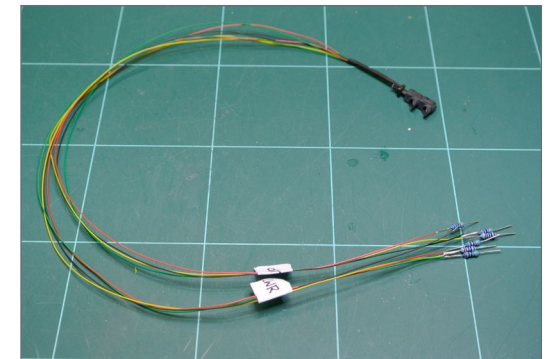
29. Completed dwarf signal with wires and resistors.
