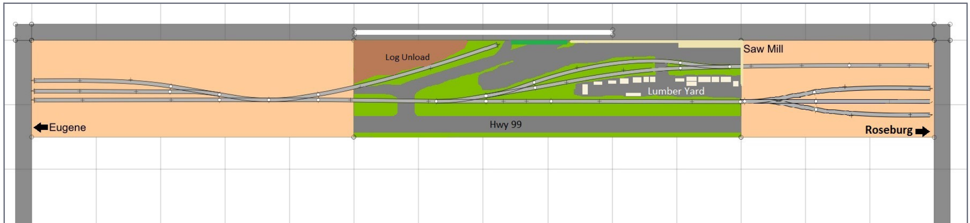
4. Initial module layout.
