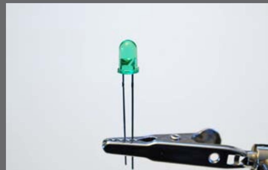
Figure 2.2: The cathode has the largest mass in an LED – another way of determining polarity.
