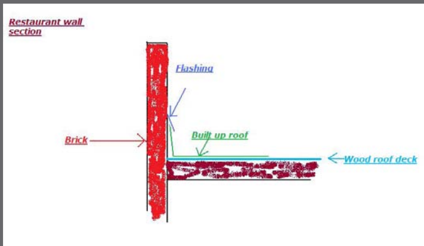
Figure 44: Drawing of flashing detail.
