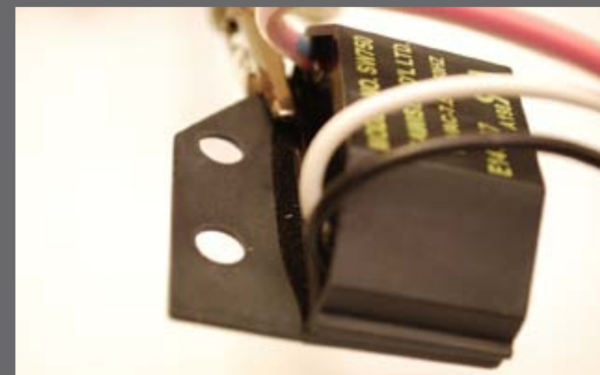
Figure 3.3: The molded bracket must be removed in order for the component to fit inside the pipe handle of the applicator.
