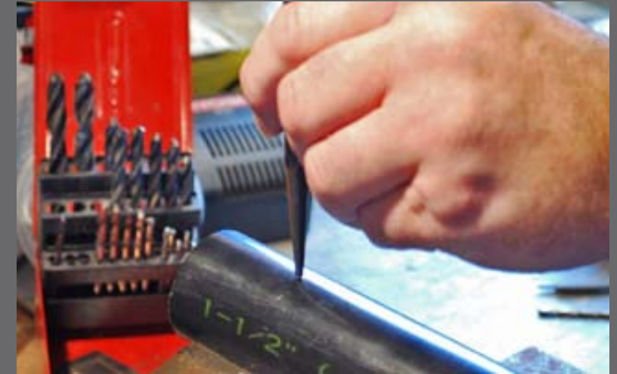
Figure 1.2: I set the cut pipe in my bench vise and used a center punch to create a centering divot to keep the drill bit from wandering.
