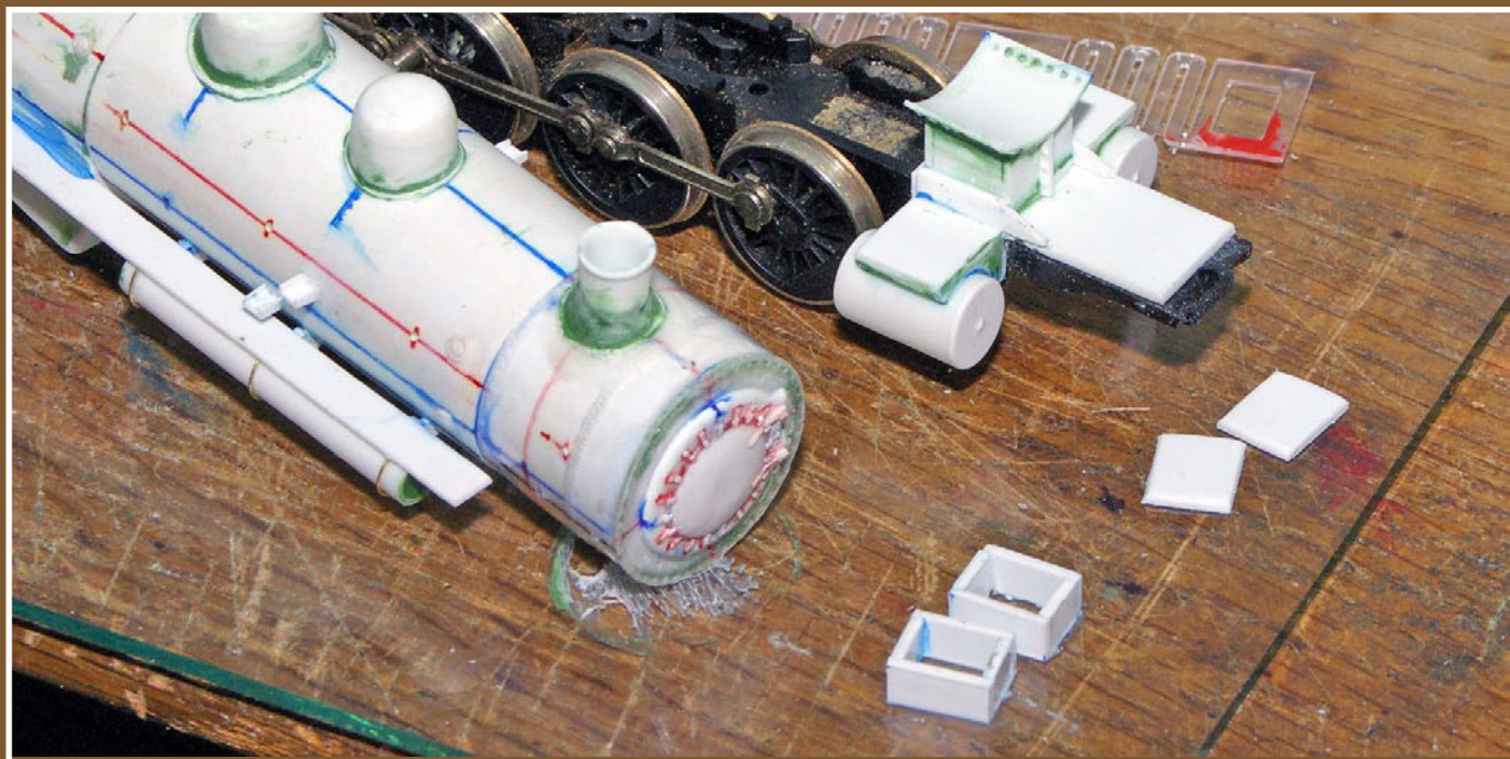
6: The steam chests are simple boxes with overhanging lids. You can also see the false upper frame members on either side of the saddle.
