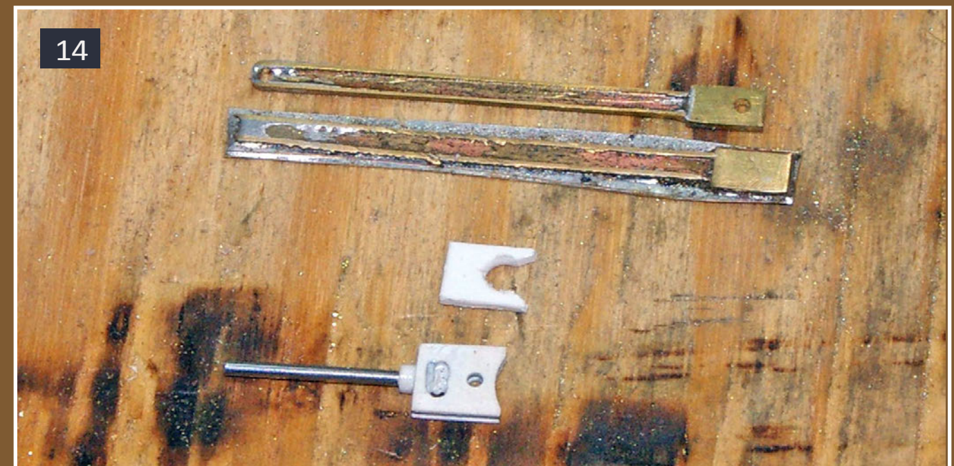
14: The crossheads and rods are built up in layers. Here you can see one of each finished along with some of the pieces that went into it.
