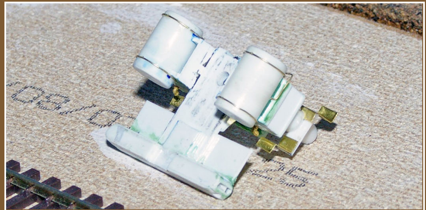
11: The underside of the pilot deck has a pad for mounting the coupler, since I chose to use a regular coupler modified to resemble those on a steam locomotive pilot.
