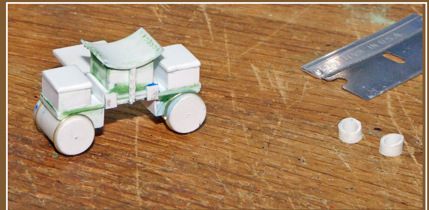
8: The little squares behind the saddle are spacers, to make it fit in the right location on the IHC frame.
