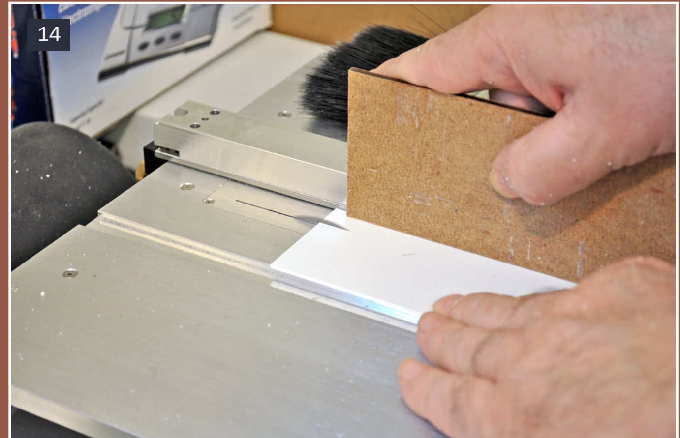
14: Once I figured out the dimensions between the rails, I cut the .040" styrene pieces.
