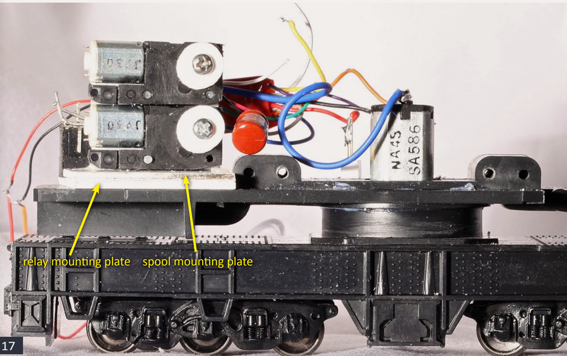
17: Mechanical assembly with cab floor, motors, relays, boom, and sound decoder.
