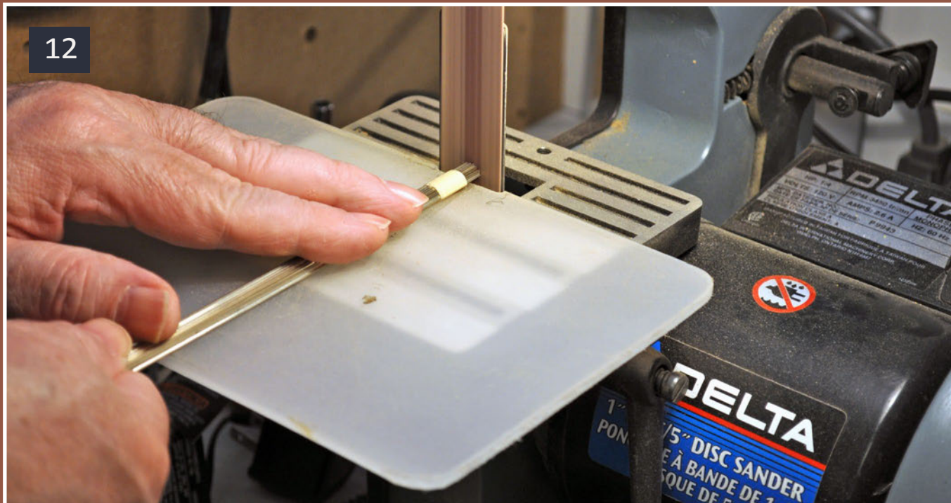
12: I taped the rails together and ground the ends to even up and to remove any burrs.
