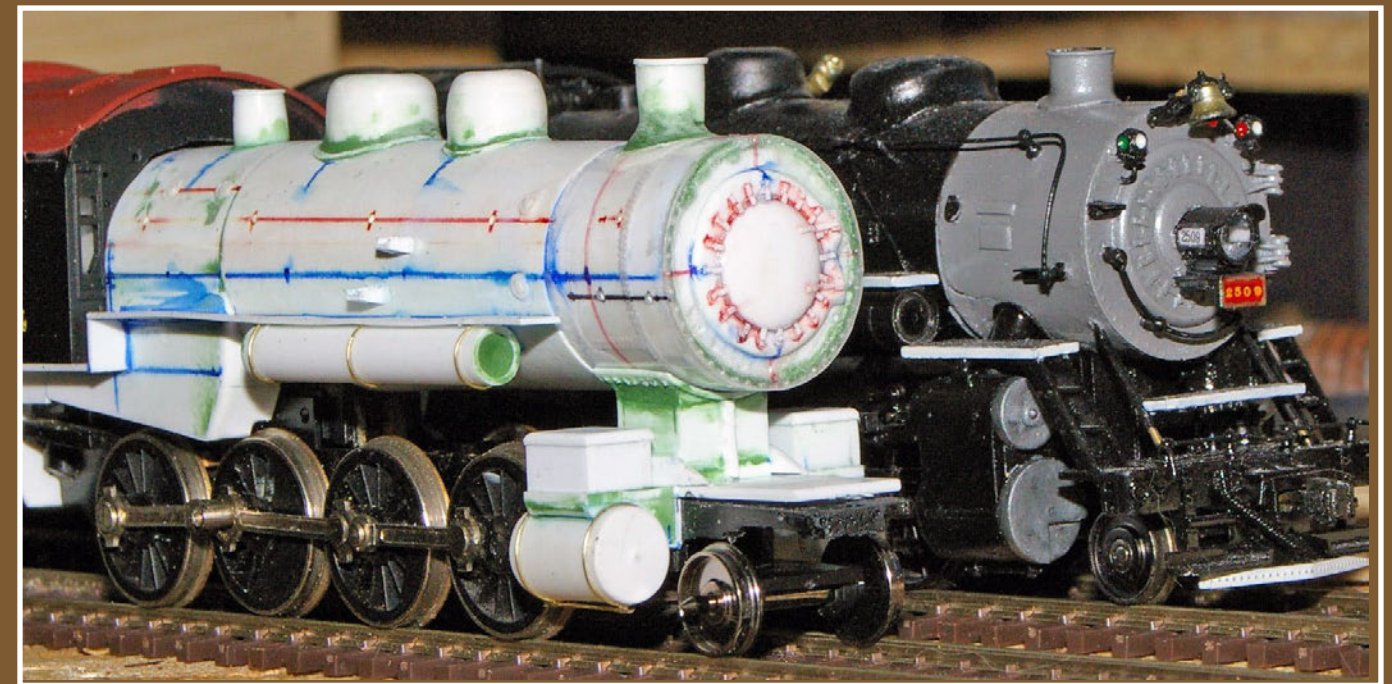
7: The brass rings simulate the rolled lip on the prototype's cylinder caps. At this point, it's a fairly accurate model of an original K class slide valve saddle.
