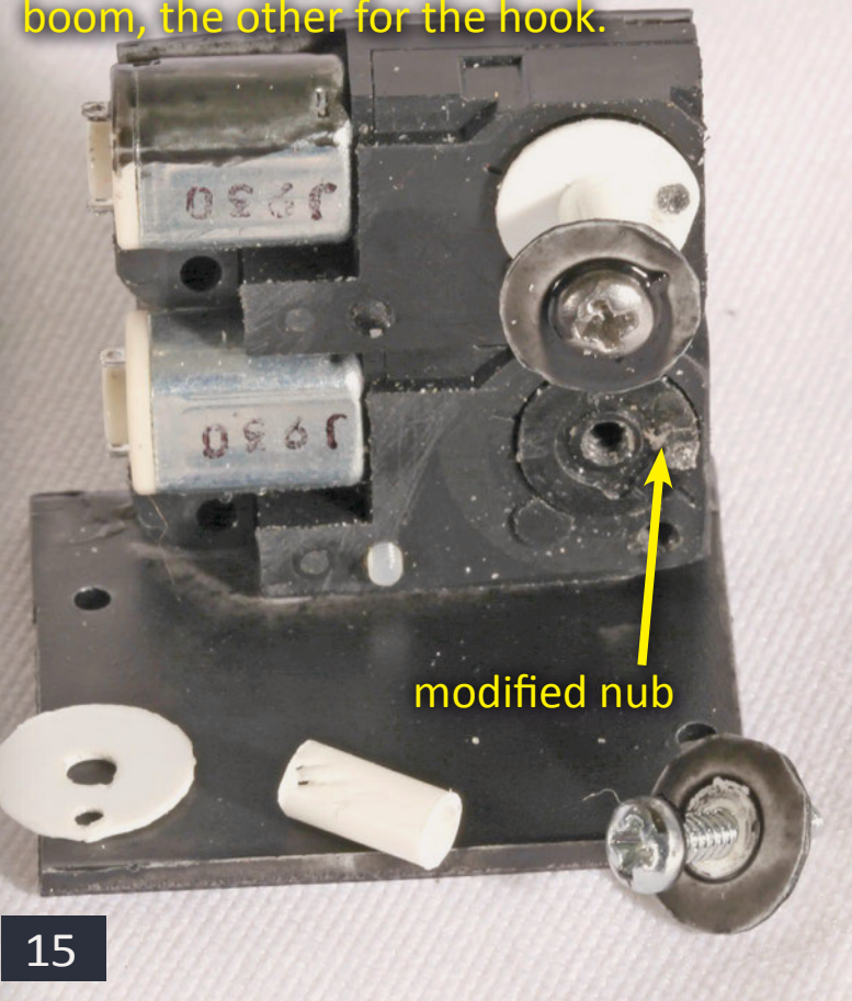
15: Drive spool parts.
