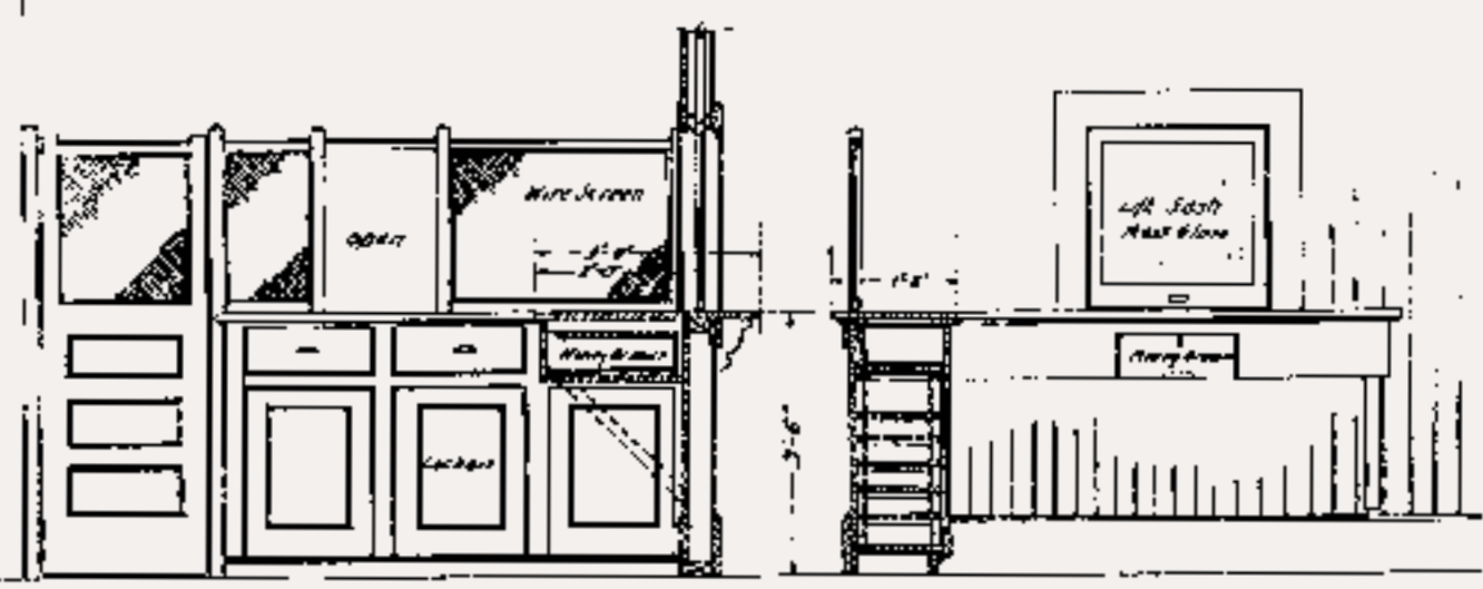
DETAIL OF COUNTER & COUNTER SHELF
