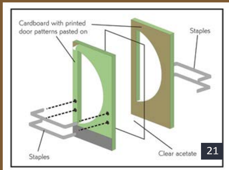
21: Door assembly.
