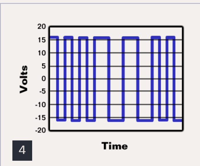
4: DCC waveform set at 16 track volts.
