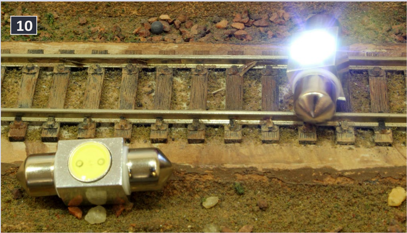
10: LED dome light testing HO track plus one off track for comparison.
