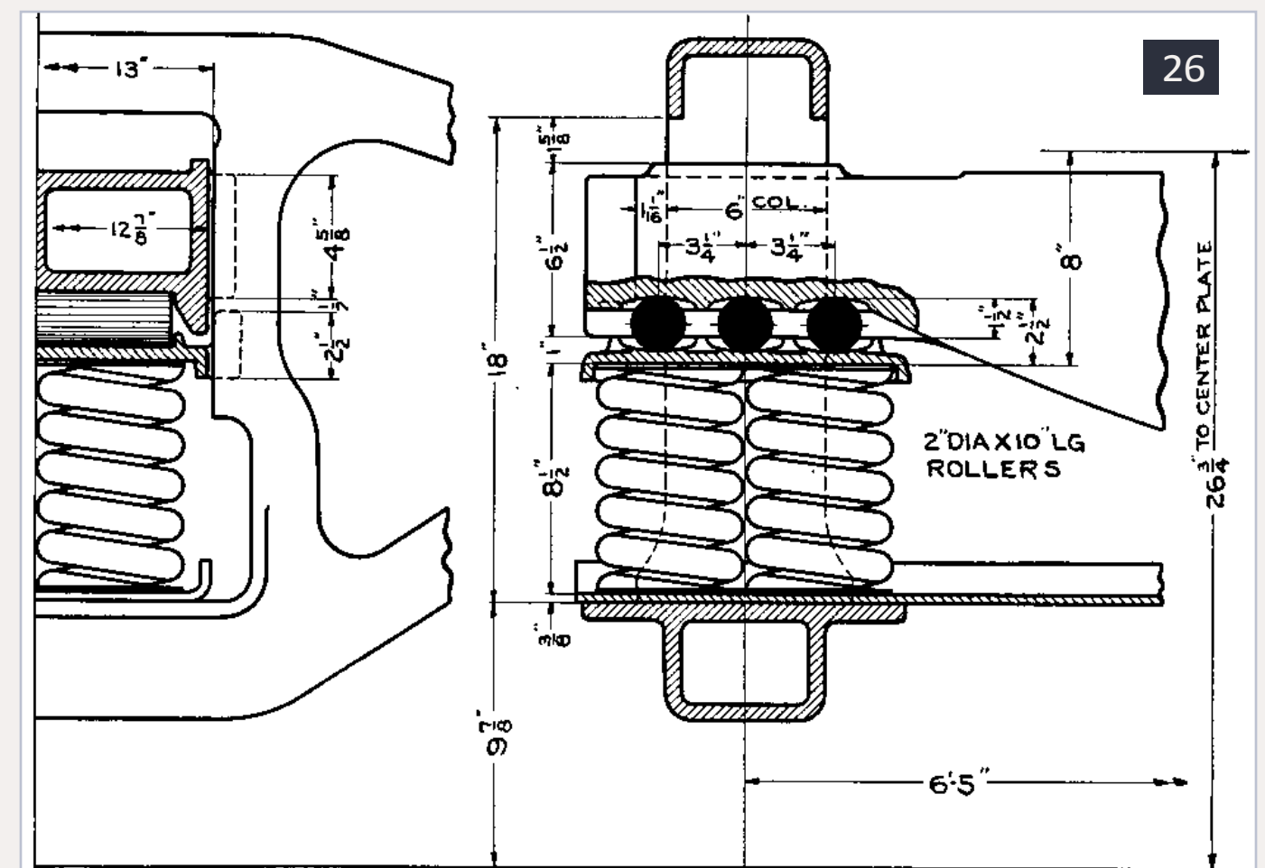
26: This cross section drawing reveals how the self-centering rollers in the Barber Lateral Motion device made limited sideways motion between the side frame and bolster possible.
