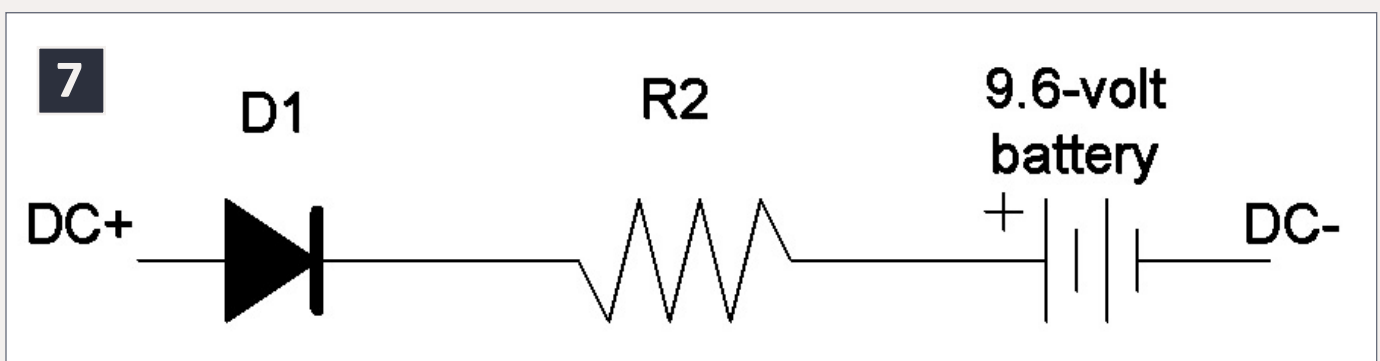
7: Battery charger circuit diagram.
