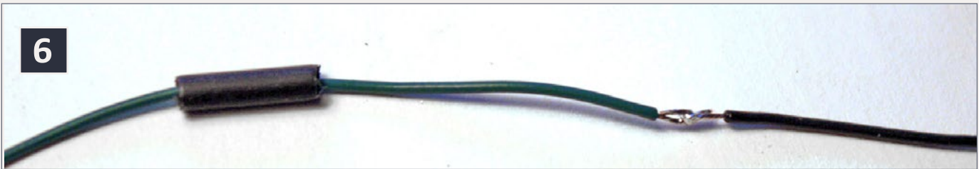
6: Soldered splice, ready for shrink tubing.
