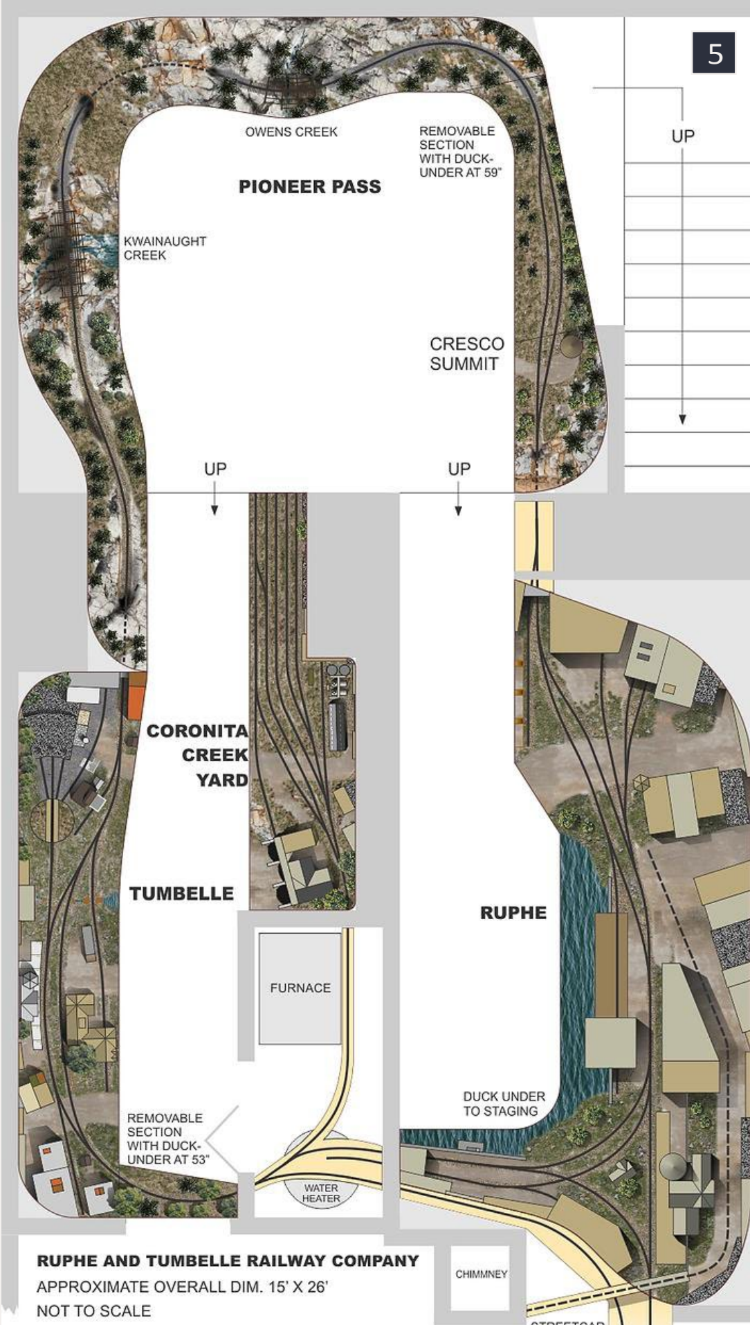
5: Rick Reimer's On30 freelanced Ruphe and Tumbelle Railway. See: mrhmag.com/track-plan-database?page=1#comment-101749
