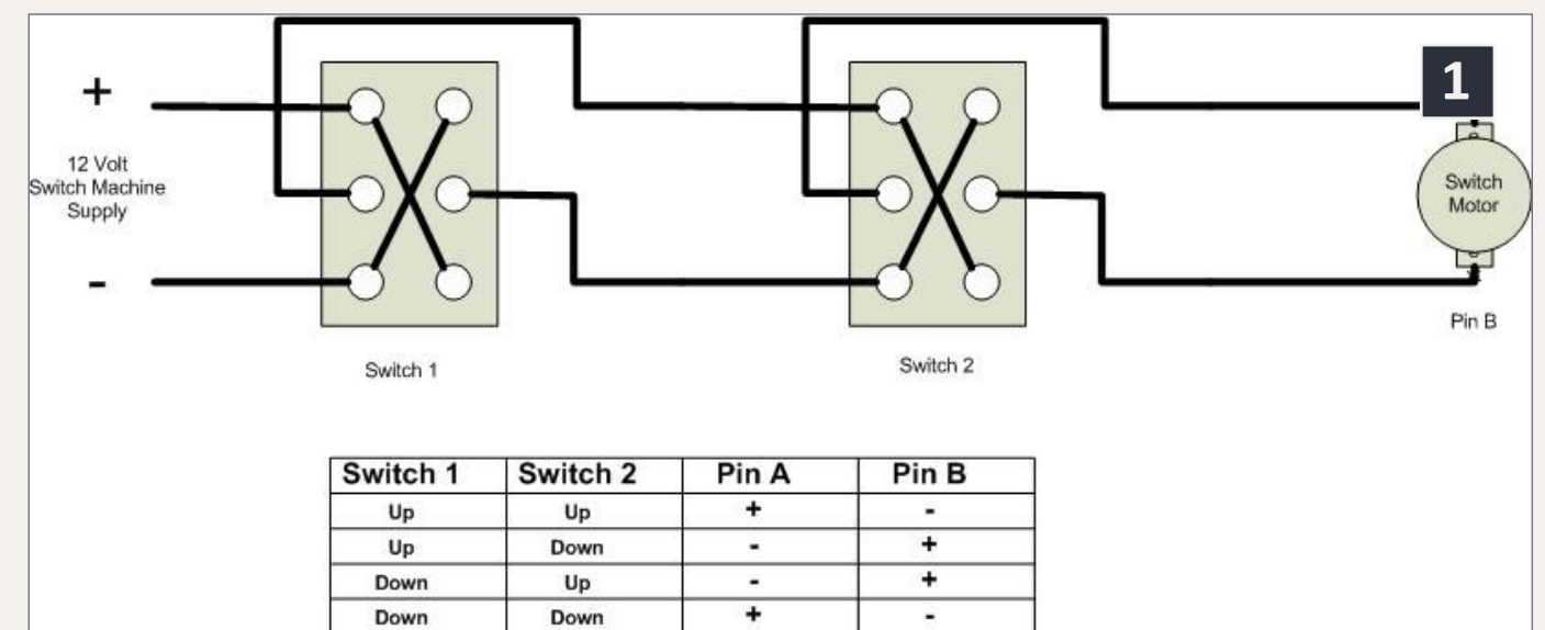
1: Rig DPDT switches to run Tortoise switch machines from more than one location. Mike Baynes diagram.
