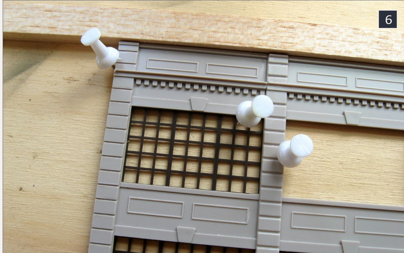
6: Push pins hold it together while I add cement. Pushing the parts together as it sets will eliminate most gaps. Any plastic that squeezes out is easily removed after it has thoroughly dried. Use a hobby knife.
