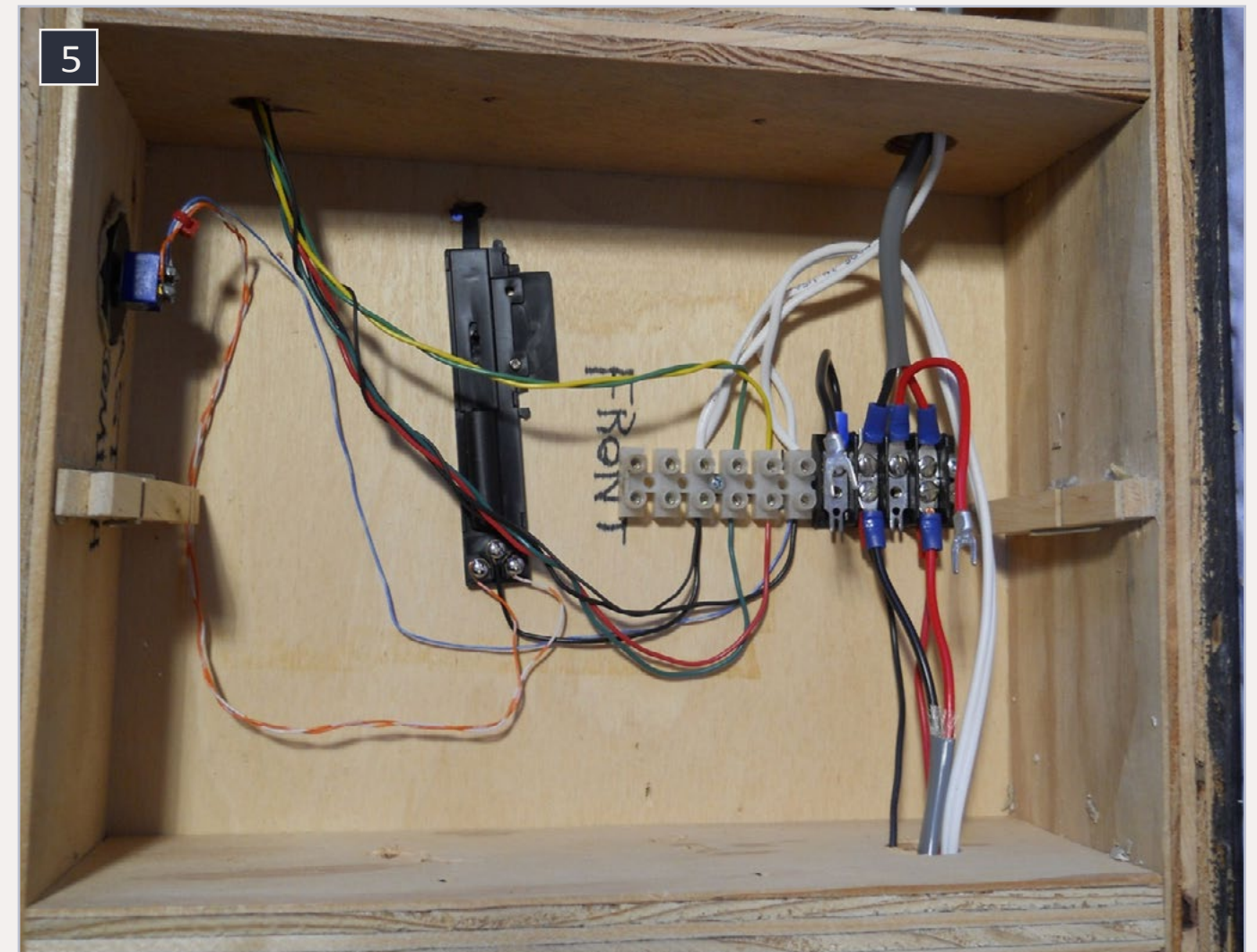
5: The power buss wiring at the right supplies electricity to the terminal strip.
