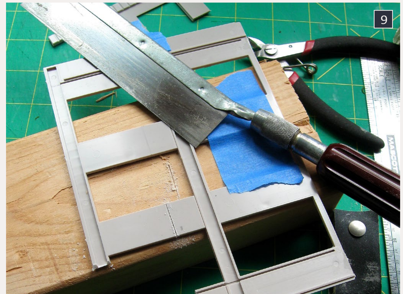
9: The rear wall was cut from behind.
