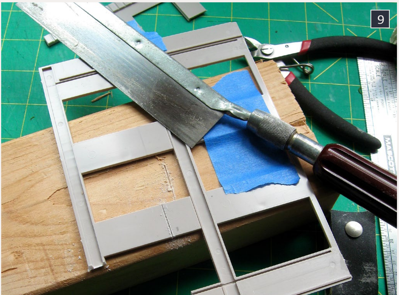
9: The rear wall was cut from behind.
