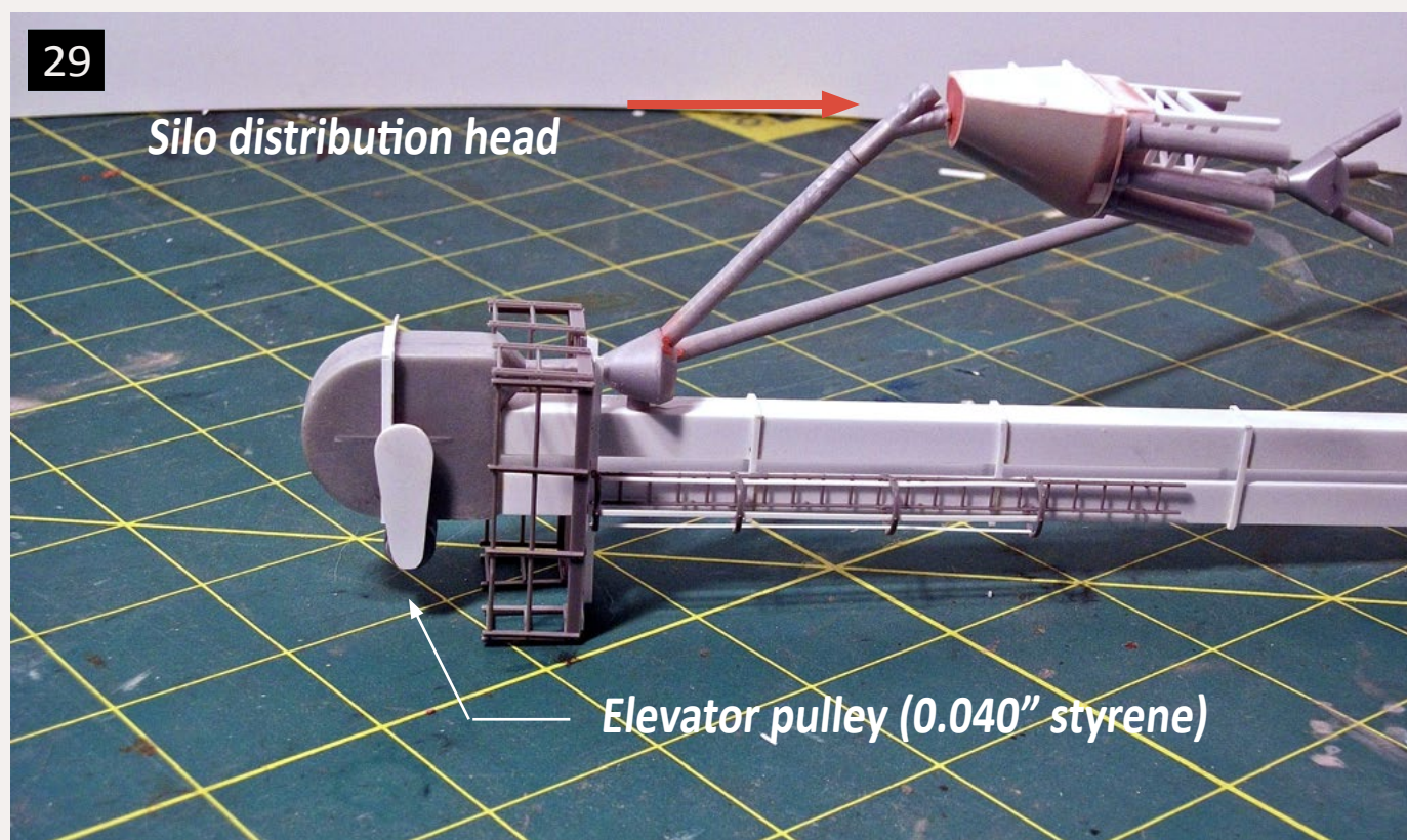
29. Partially completed feed bin elevator and distribution head. The unpainted photo illustrates the general construction of the elevator, head assembly and pulley guard along with handrails, distributor, and Rix Products piping.
