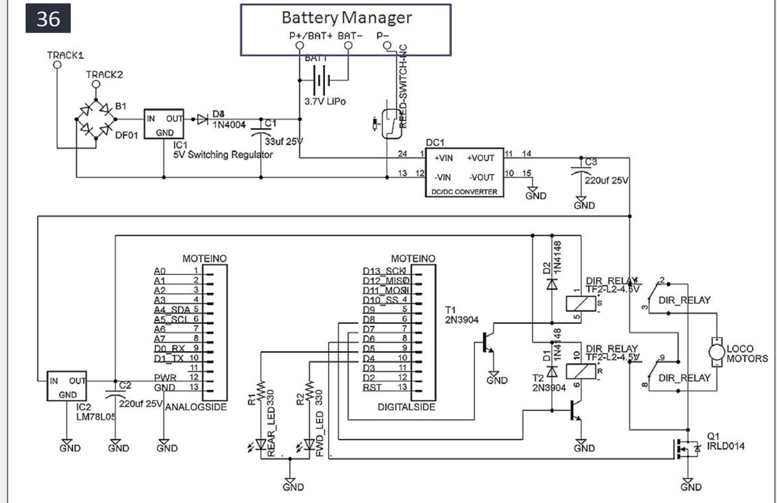
36. Locomotive higher power schematic.
