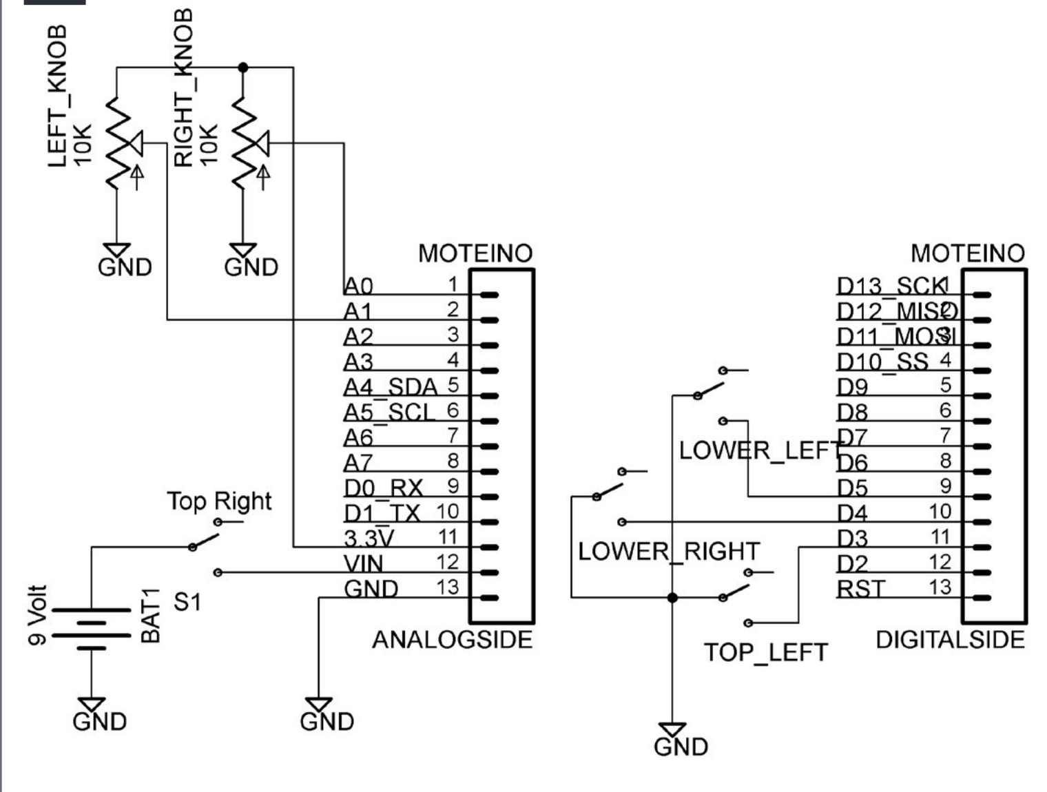
34. Loco controller schematic.
