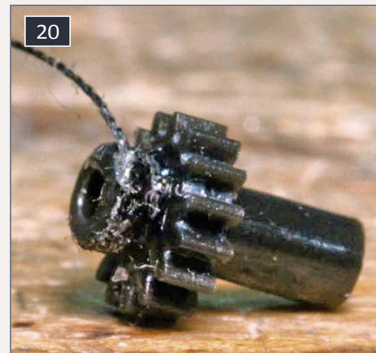
20. Repairing gears.
