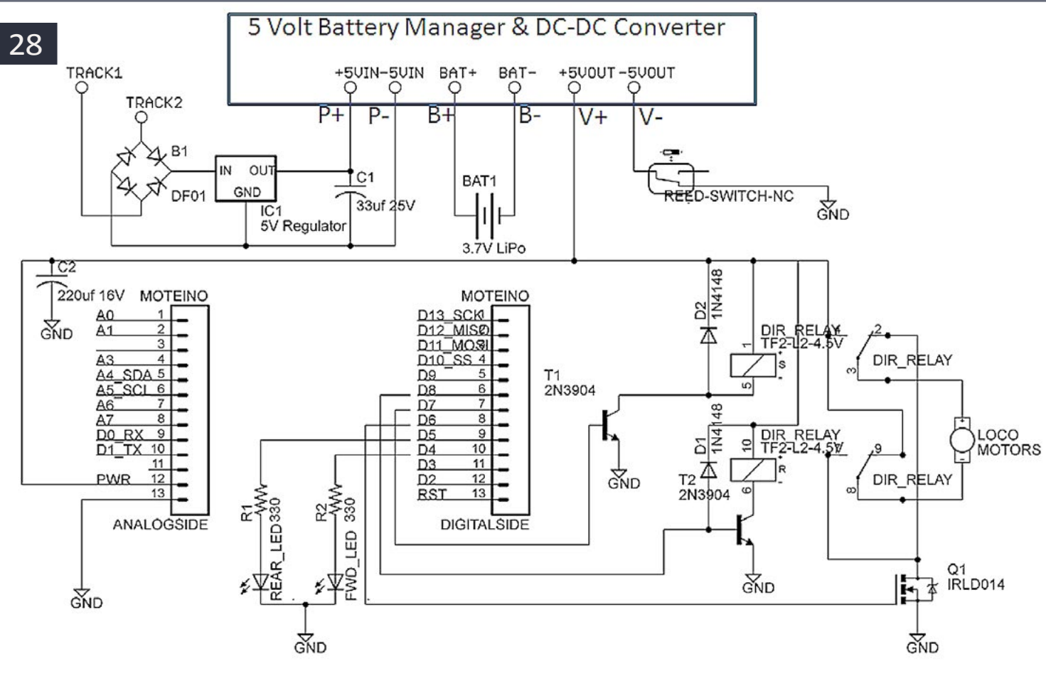
28. Locomotive battery power block diagram.
